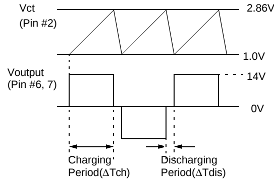
Figure 2. Oscillator sawtooth & Output gate drive waveform
