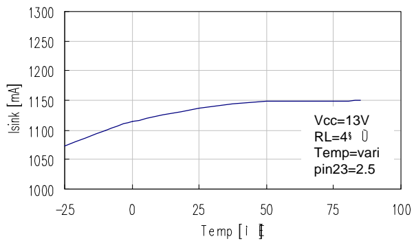
Temp vs. I_{SINK}
