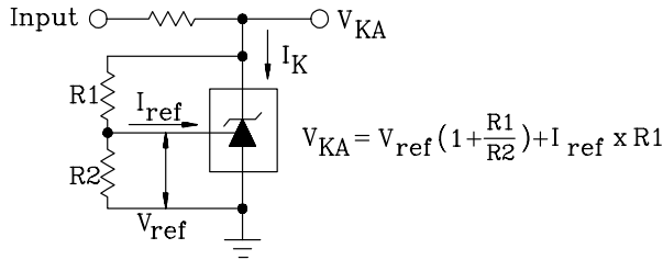
FIGURE 2—TEST CIRCUIT FOR V_{KA} > V_{ref}
