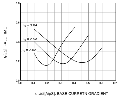
Figure 10. Switching Characteristic
