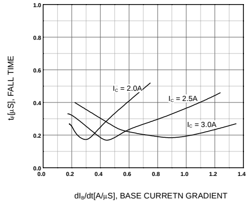
Figure 8. Switching Characteristic
