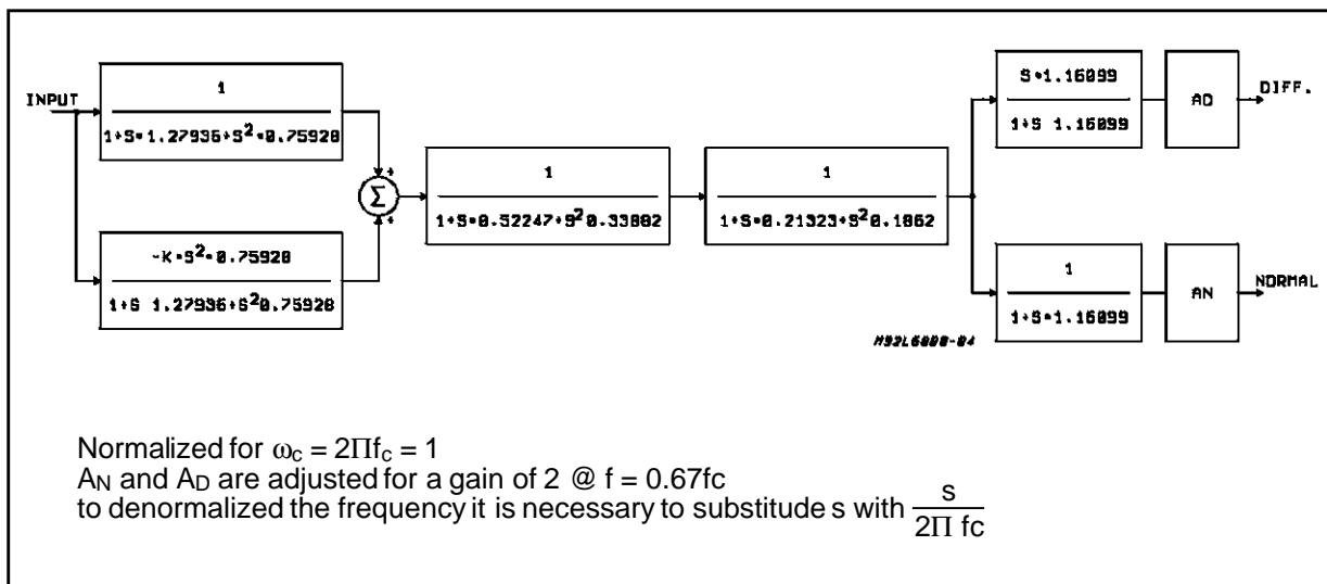
Figure 2: Normalized block diagram for filter
