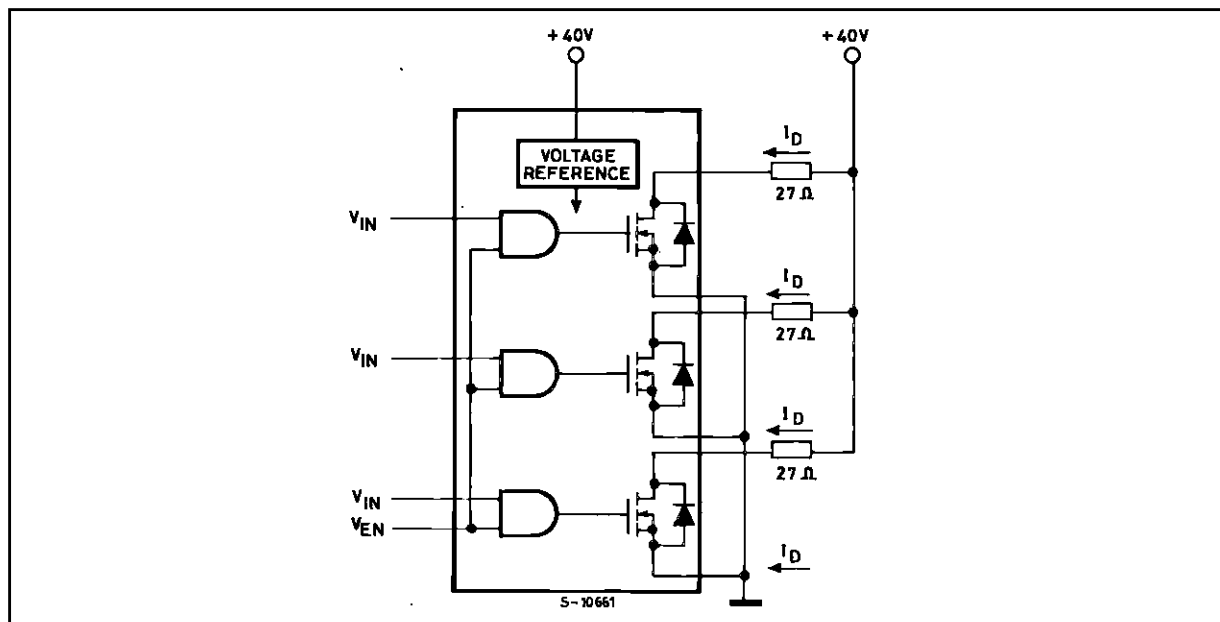
Figure 1 : Test Circuit.
