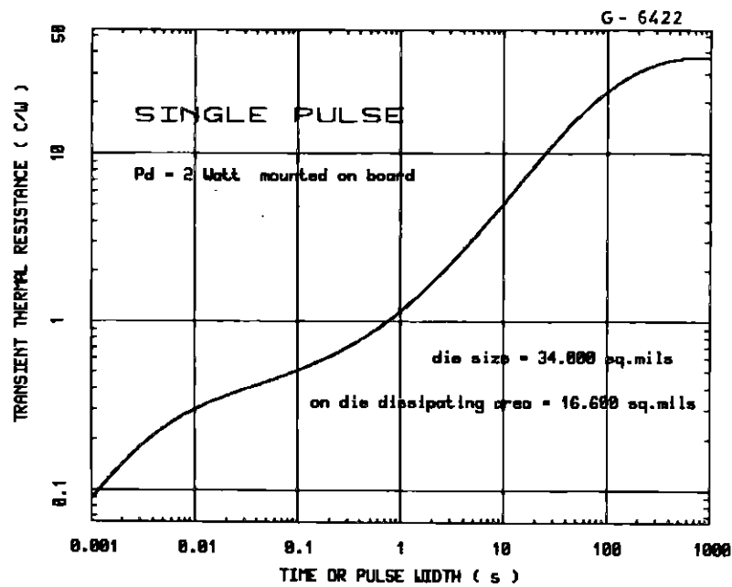
Figure 8 : Transient Thermal Resistance for Single Pulses (Multiwatt).
