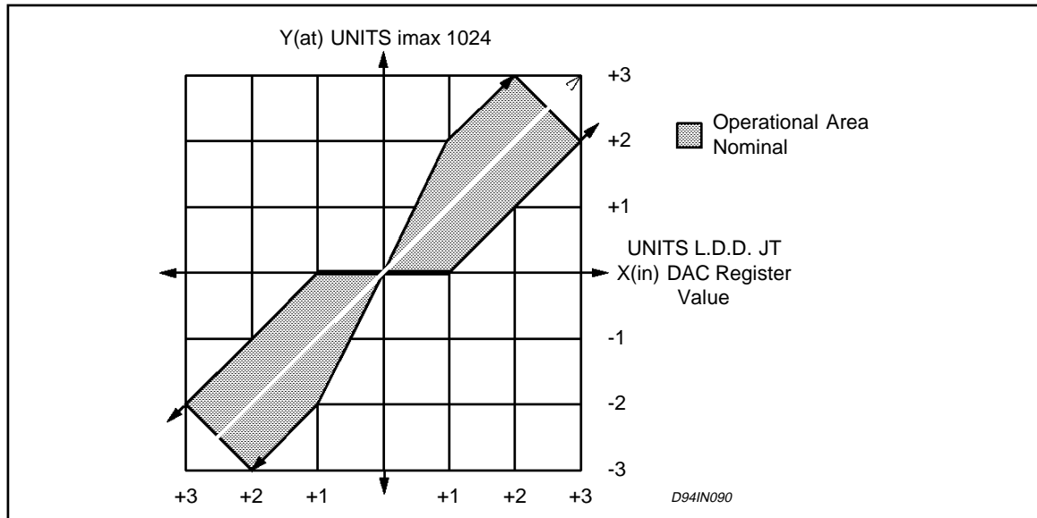
Figure 1: V_{jump} vs. Deadband
