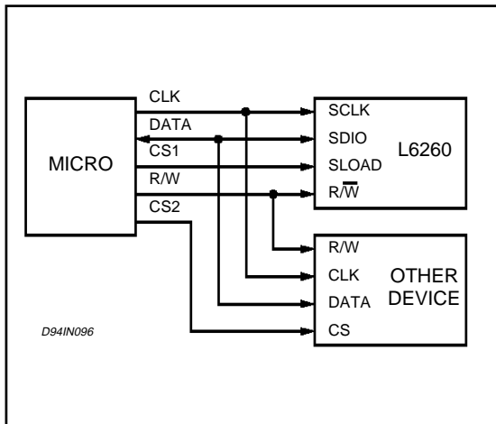
Figure 7: System Level Interface
