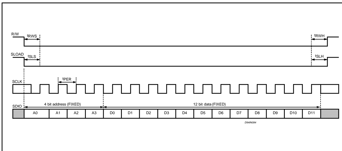
Figure 5: Serial Write Timing Diagram
