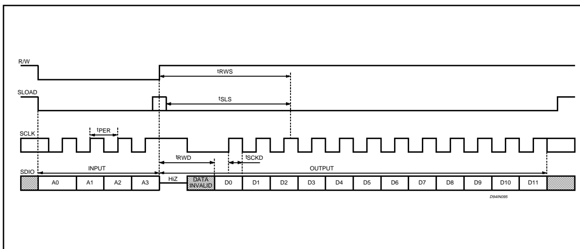
Figure 6: Serial Read Timing Diagram
