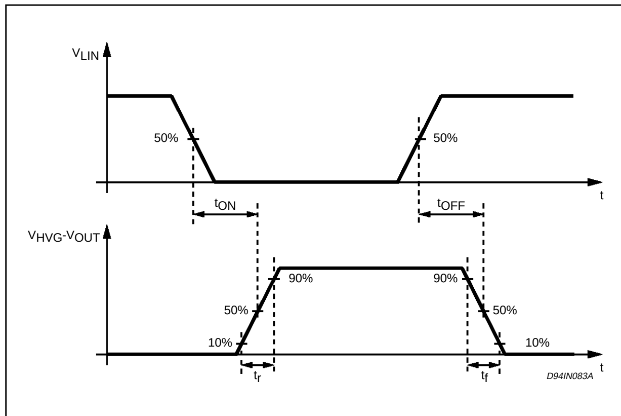
Figure 2: Switching Waveforms
