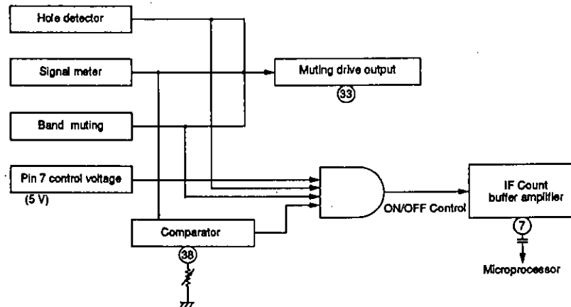
Figure 8. IF count buffer
