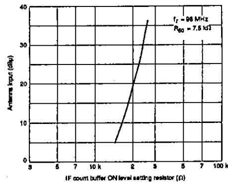
Figure 17. Antenna input vs. IF count buffer ON threshold resistance
