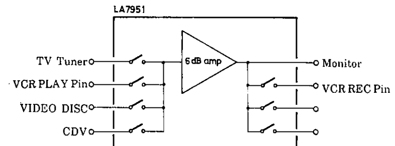
Figure 2. Video Selector Switch Connections
