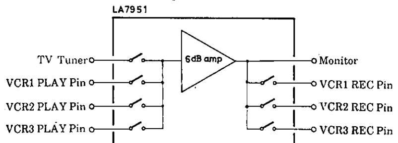
Figure 1. Editing System Switch Connections
