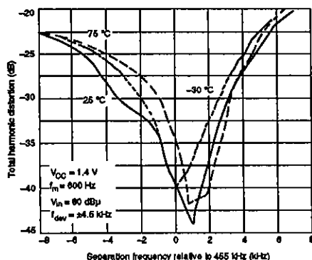
Tuning characteristics
