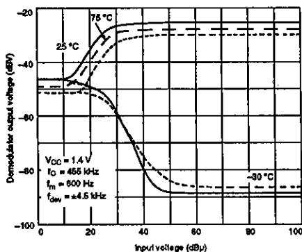
Tuning characteristics
