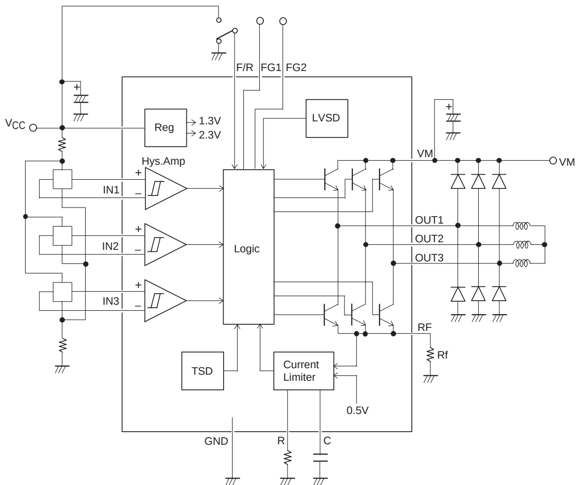
Block Diagram and Peripheral Circuitry
