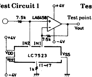
Test Circuit 1
