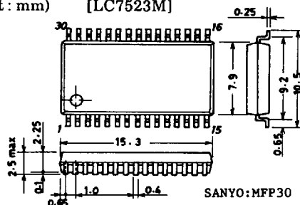
Case Outline 3073A (unit : mm) [LC7523M]
