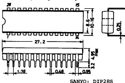
Case Outline 3029A (unit : mm) [LC7523]
