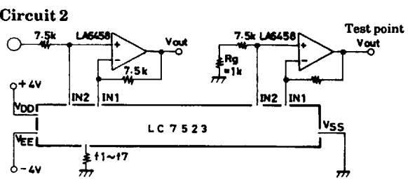
Test Circuit 2
