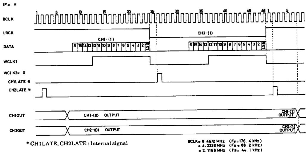
Timing Chart 1
