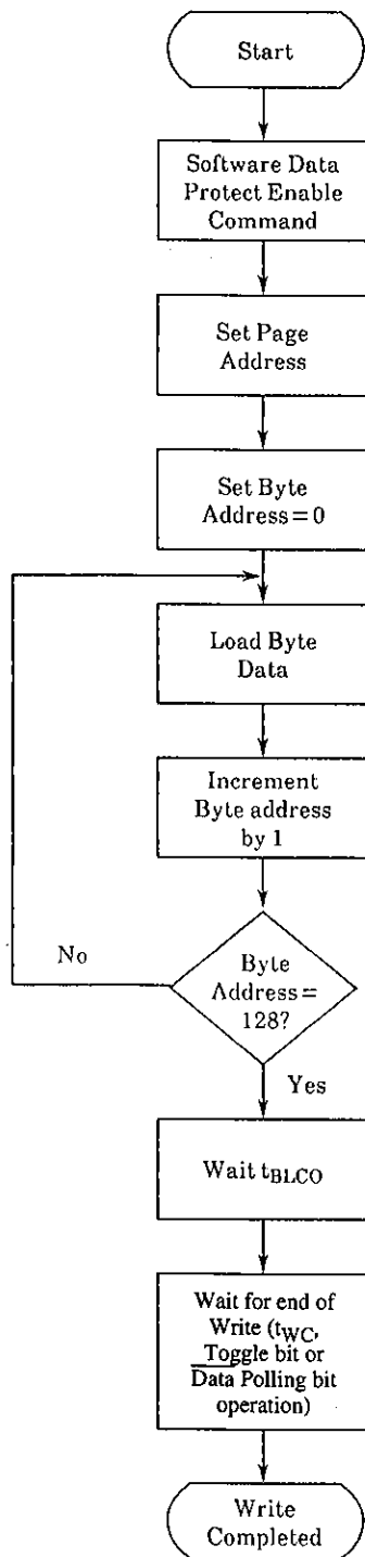
Figure 10 Write Algorithm
