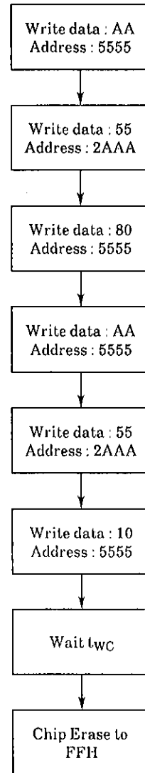
Figure 14 Software Chip-Erase Flowchart
