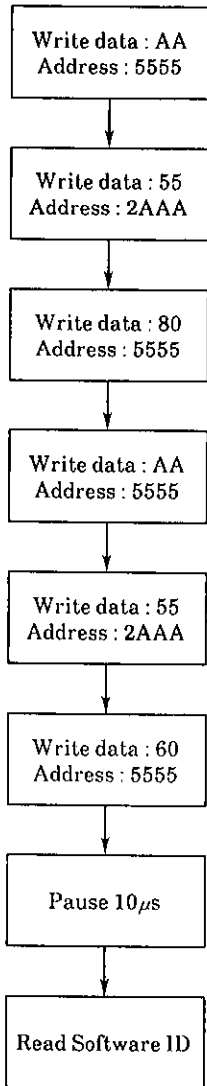
Figure 13 Product ID Flowcharts
