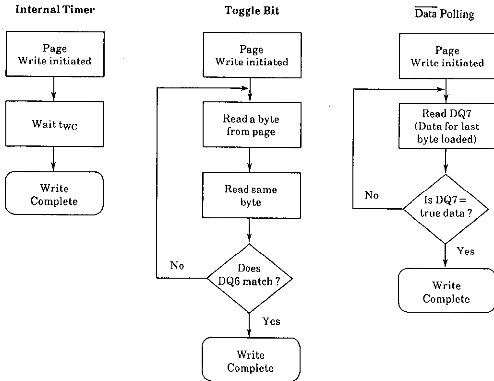
Figure 11 Write Operating State Detection
