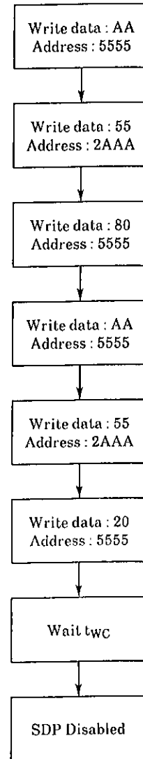
Figure 12 Software Data Protection Flowcharts
