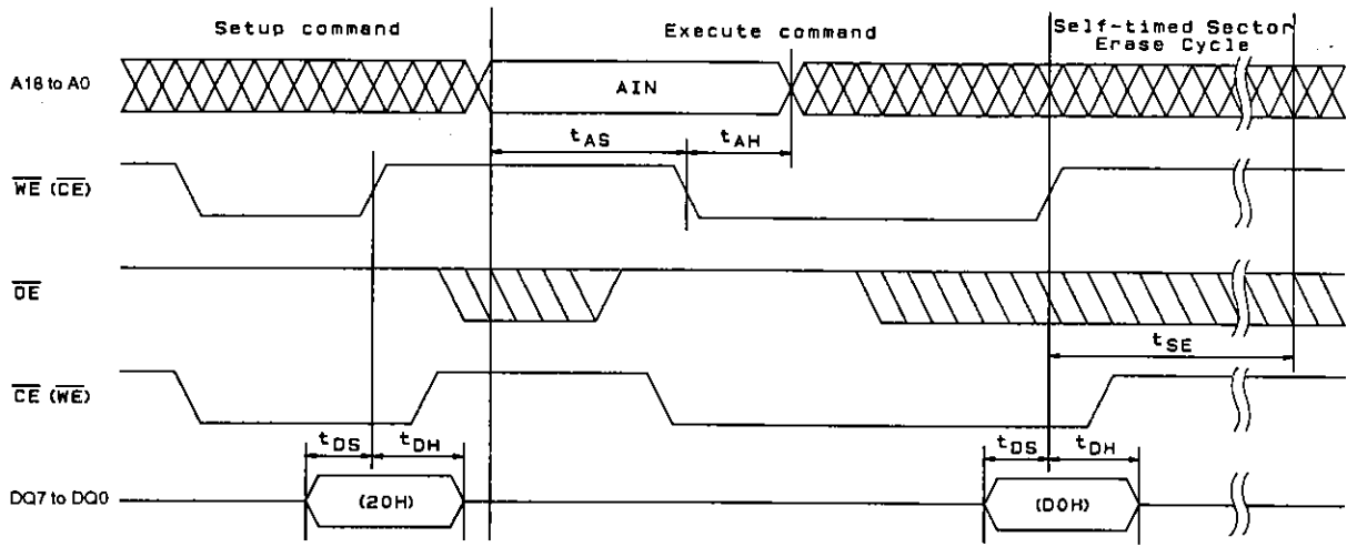
Figure 6 Sector Erase
