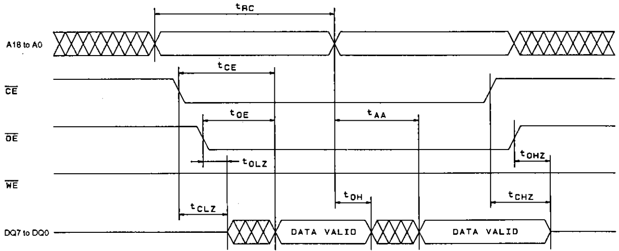
Figure 3 Read Cycle
