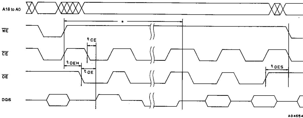
Figure 12 Toggle Bit (DQ6)
