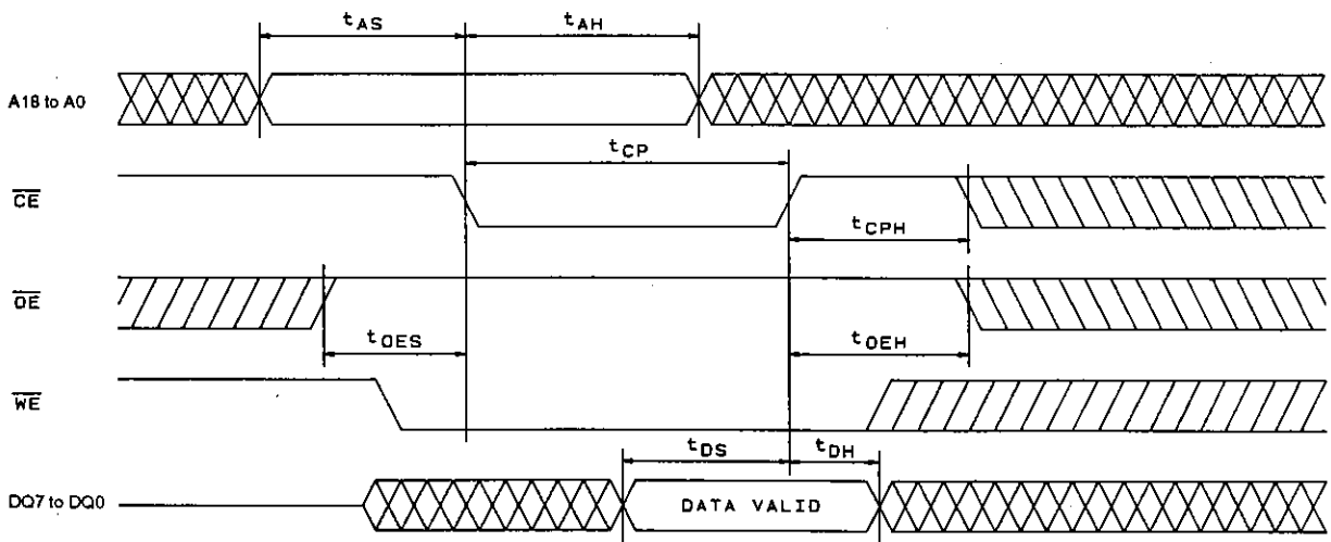
Figure 4 WE Control Write Cycle
