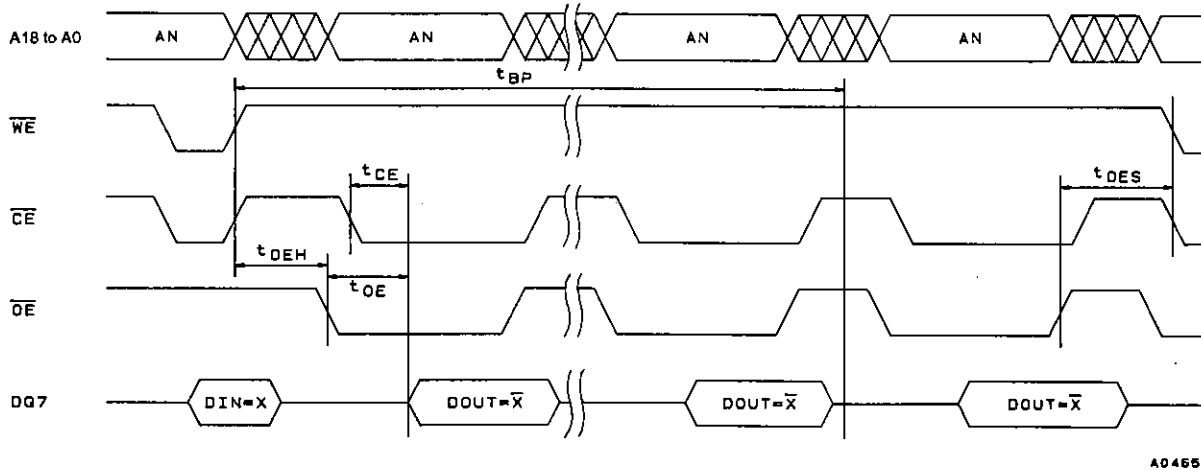
Figure 11 Data polling(DQ7)
