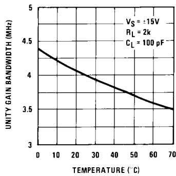
Gain Bandwidth
