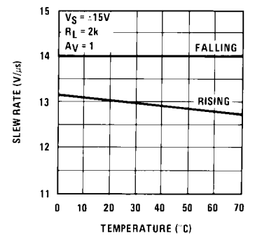
Slew Rate
