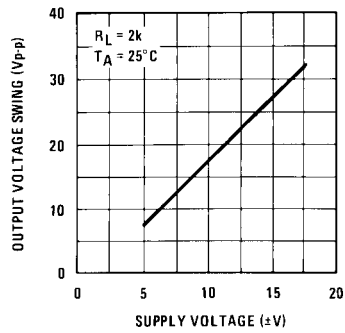
Voltage Swing
