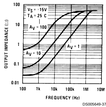
Output Impedance
