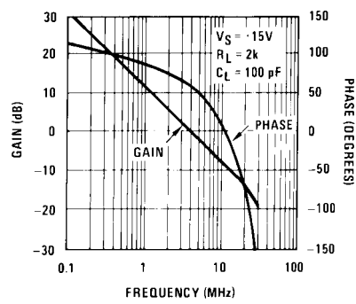
Bode Plot
