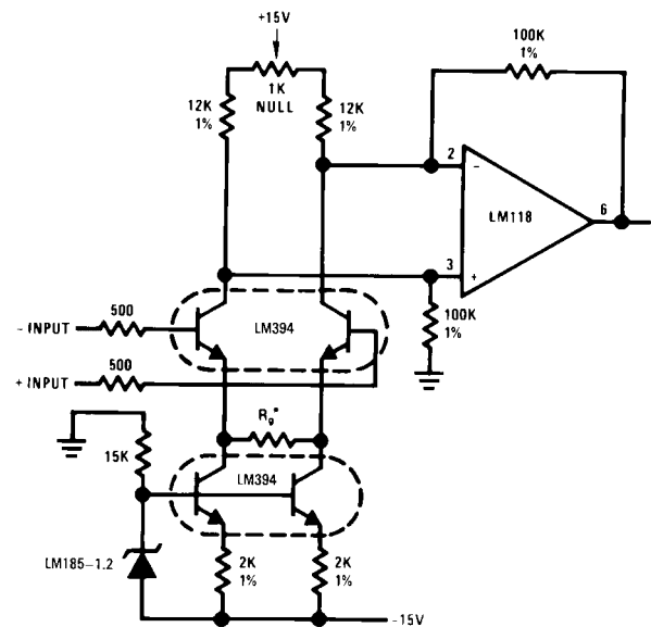
Instrumentation Amplifier
