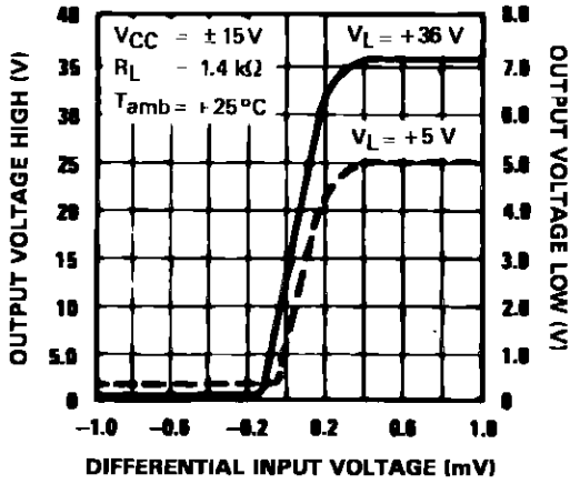
TRANSFER FUNCTION
