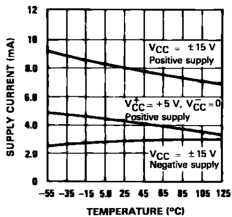
SUPPLY CURRENT
