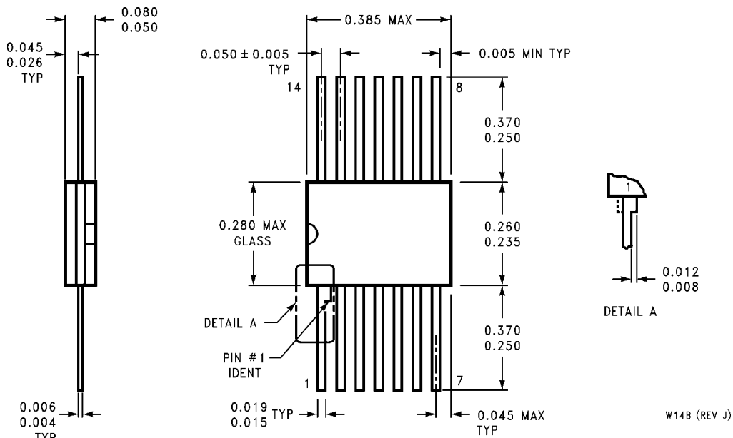
Ceramic Flatpak Package Order Number JL124ABDA, JL124ABZA, JL124ASDA, JL124BDA, JL124BZA, JL124SDA, LM124AW/883, LM124WG/883, LM124W/883 or LM124WG/883 NS Package Number W14B
