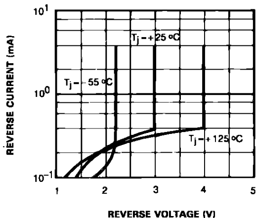
REVERSE CHARACTERISTICS
