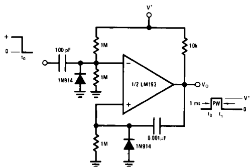
One-Shot Multivibrator
