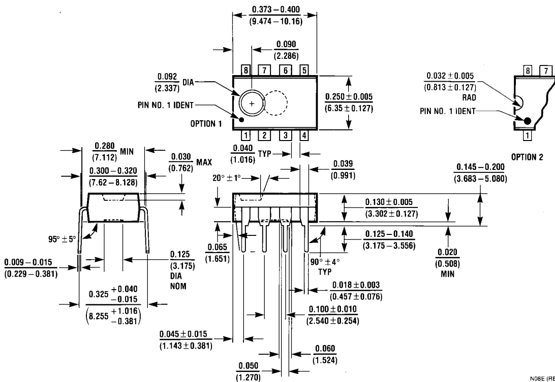
Molded Dual-In-Line Package (N) Order Numbers LM393N or LM2903N NS Package N08E
