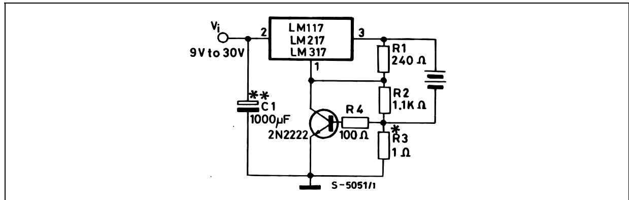
Figure 11 : Current Limited 6V Charger
