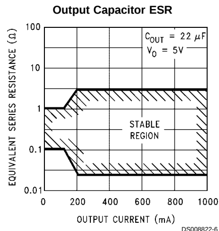
FIGURE 1. ESR Limits
