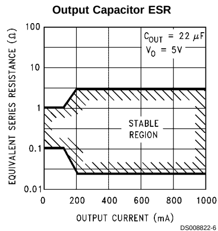
FIGURE 1. ESR Limits
