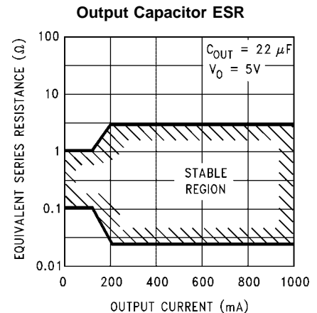
FIGURE 1. ESR Limits
