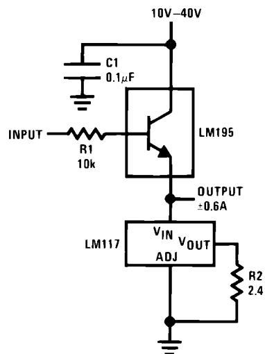
Power Follower
