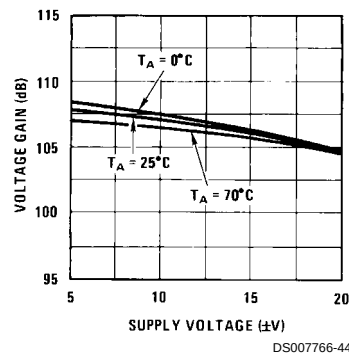
Voltage Gain
