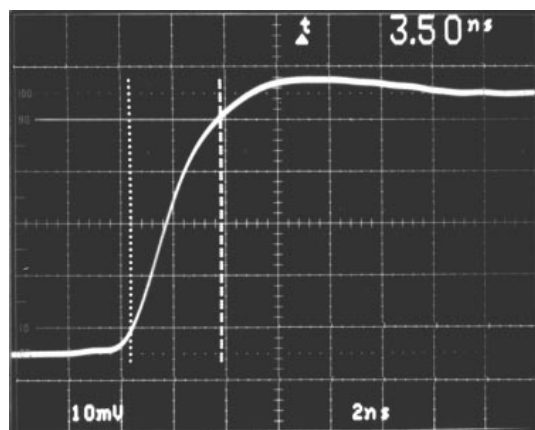
Current Feedback Amp Small-Signal Response V_S = \pm 15V , R_F = 750\Omega , R_L = 100\Omega
