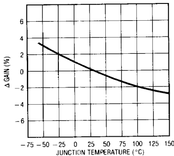
Current Sense Amplifier Gain vs Temperature
