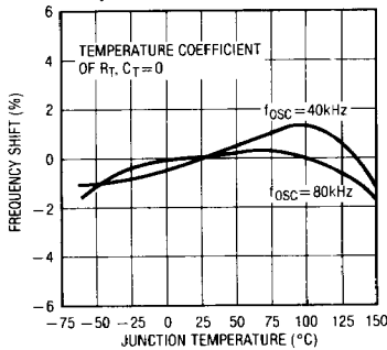
Oscillator Frequency vs Temperature
