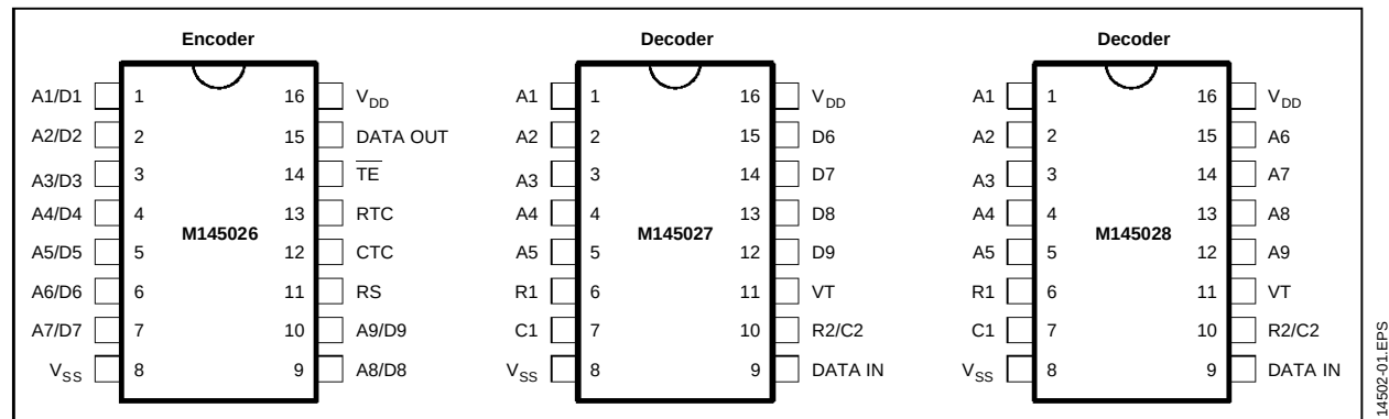
Figure 1 : Encoder M145026
