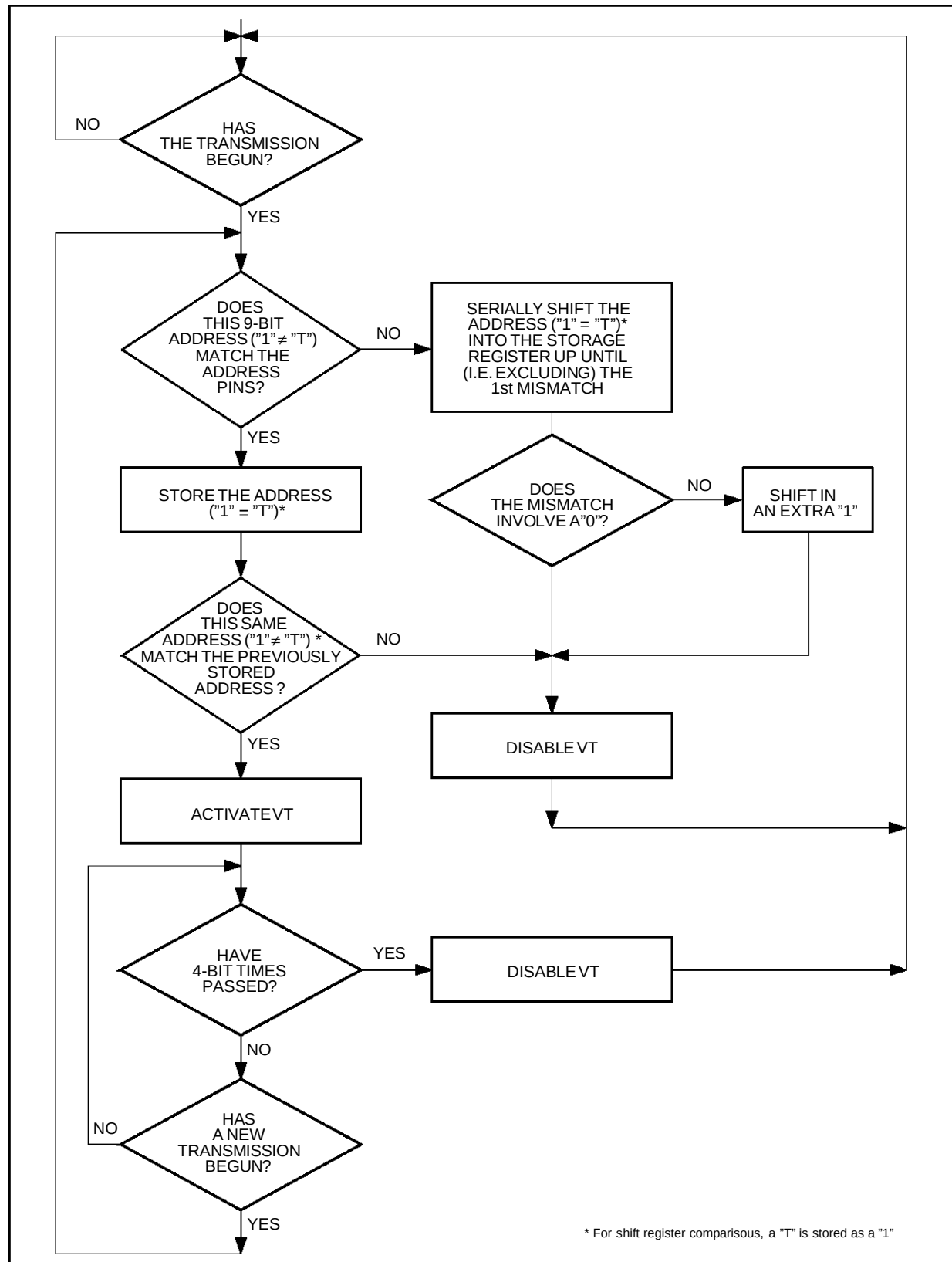
Figure 8 : M145028 Flowchart
