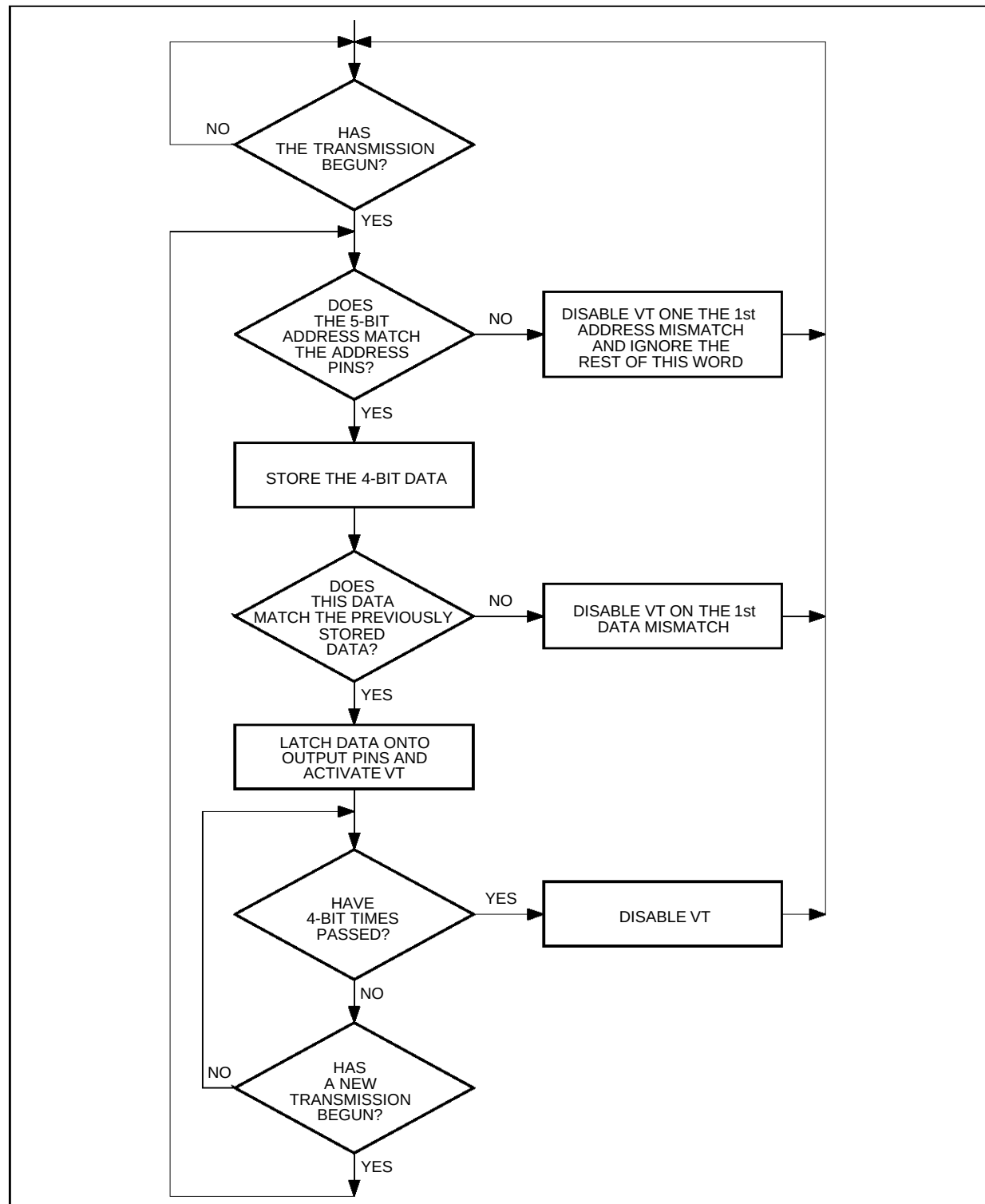
Figure 7 : M145027 Flowchart
