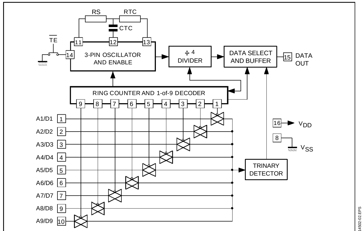
Figure 1 : Encoder M145026
