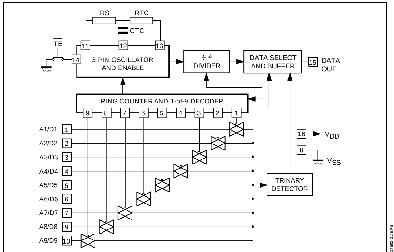
Figure 1 : Encoder M145026
