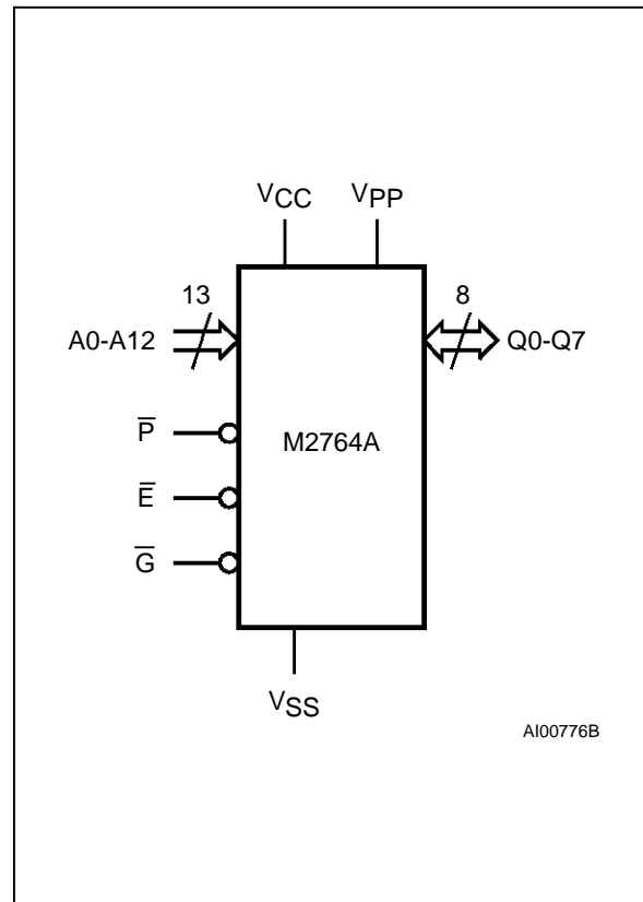
Figure 1. Logic Diagram
