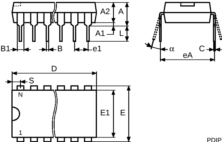
PDIP
