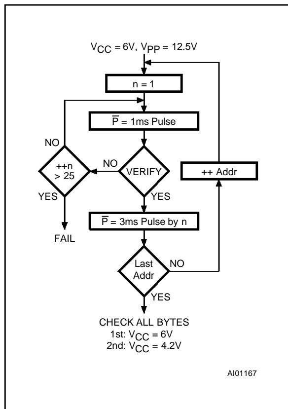
Figure 7. Programming Flowchart
