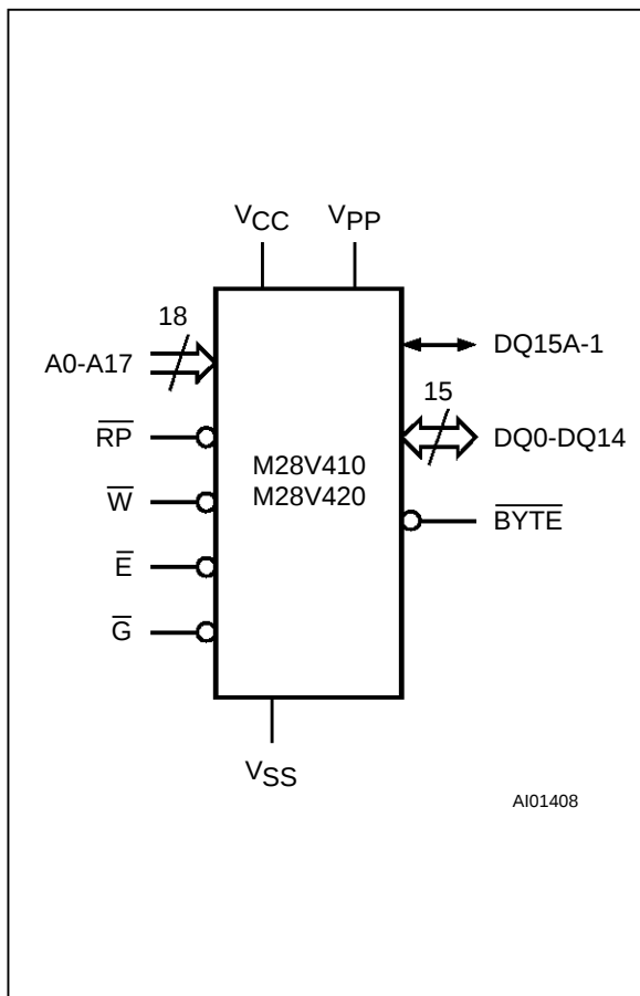
Figure 1. Logic Diagram
