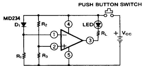
(3) Battery check circuit
