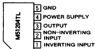
Outline 5P5T
