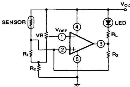
(2) Sensor detection circuit
