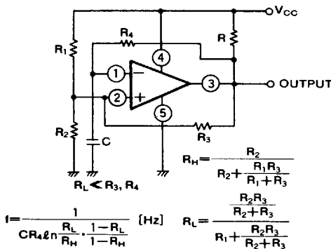
(4) Oscillator
