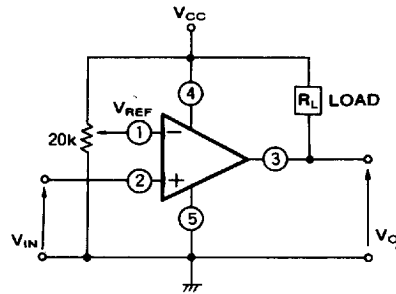
(1) Voltage comparator
