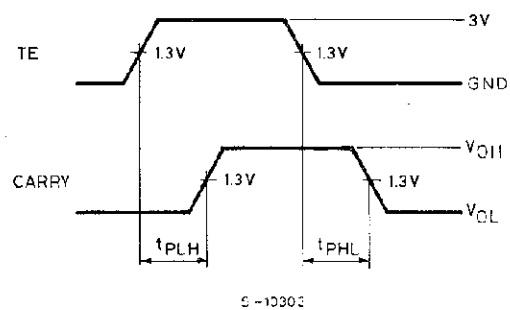
CASCADE MODE (fix maximum count)
