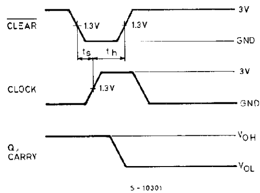
CLEAR MODE (HCT162/163)
