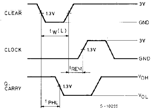
CLEAR MODE (HCT160/161)
