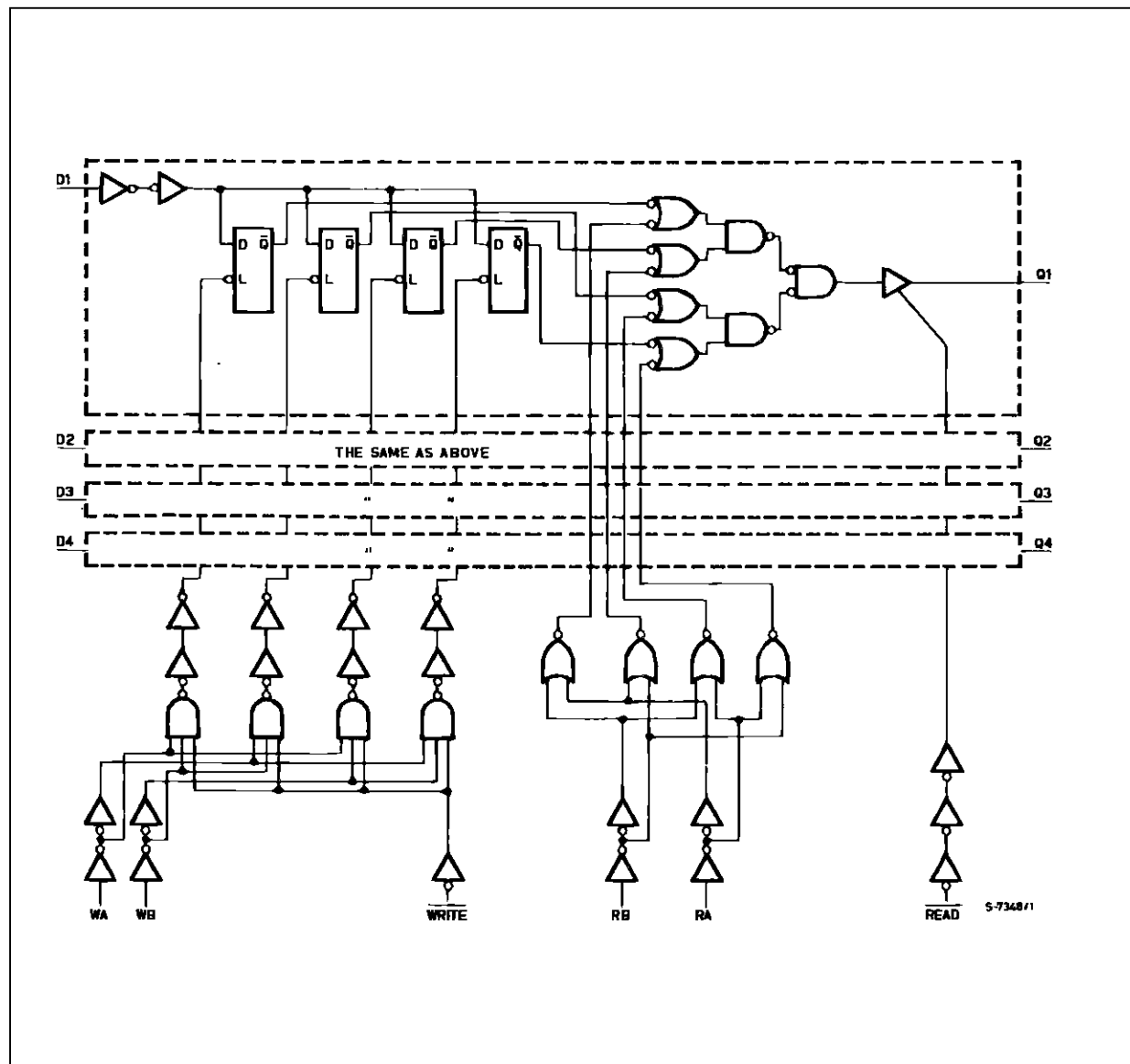
LOGIC DIAGRAM
