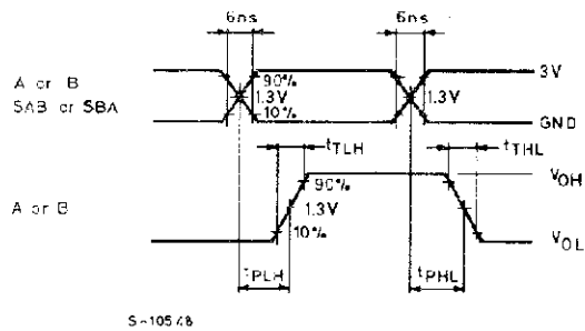
WAVEFORM 1
