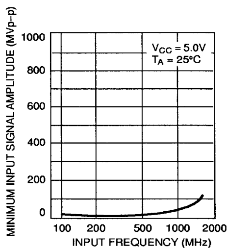
Figure 2. Input Signal Amplitude vs. Input Frequency
