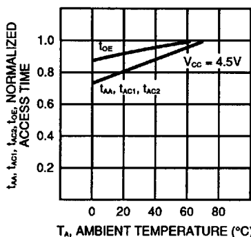
Fig. 8 - NORMALIZED ACCESS TIME vs. AMBIENT TEMPERATURE
