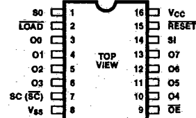
Plastic SOP (Suffix -PF) FPT-16P-M02
