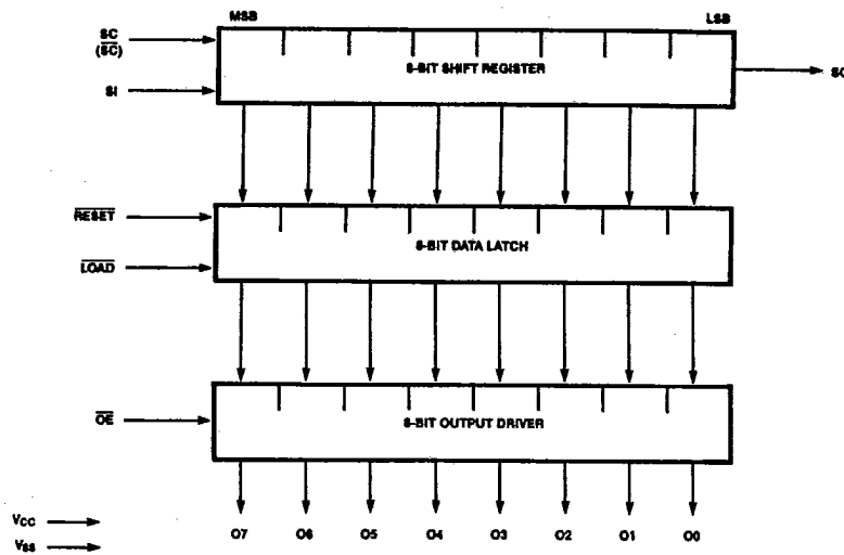
Figure 1. Block Diagram
