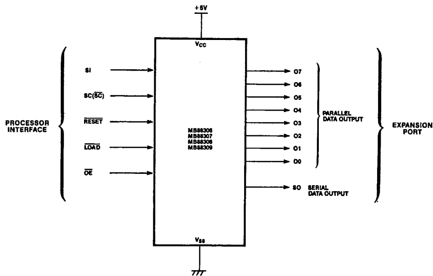
Figure 2. System Interface
