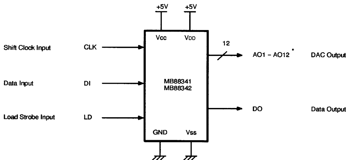
Figure 1 Logic Symbol
