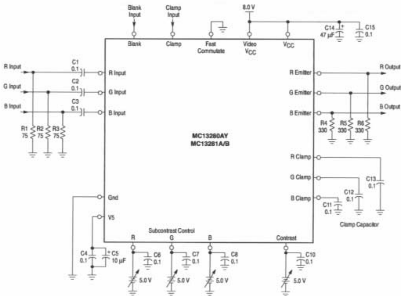
Figure 2. Test Circuit
