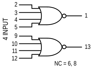
MC14002B Dual 4-Input NOR Gate
