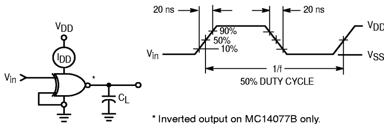
Figure 1. Power Dissipation Test Circuit and Waveform
