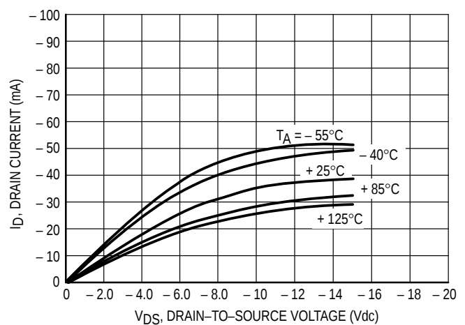
Figure 7. V_{GS} = -15 Vdc
