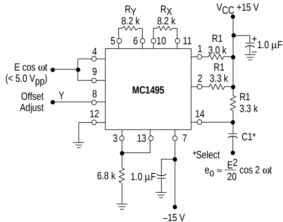
Figure 28. Frequency Doubler
