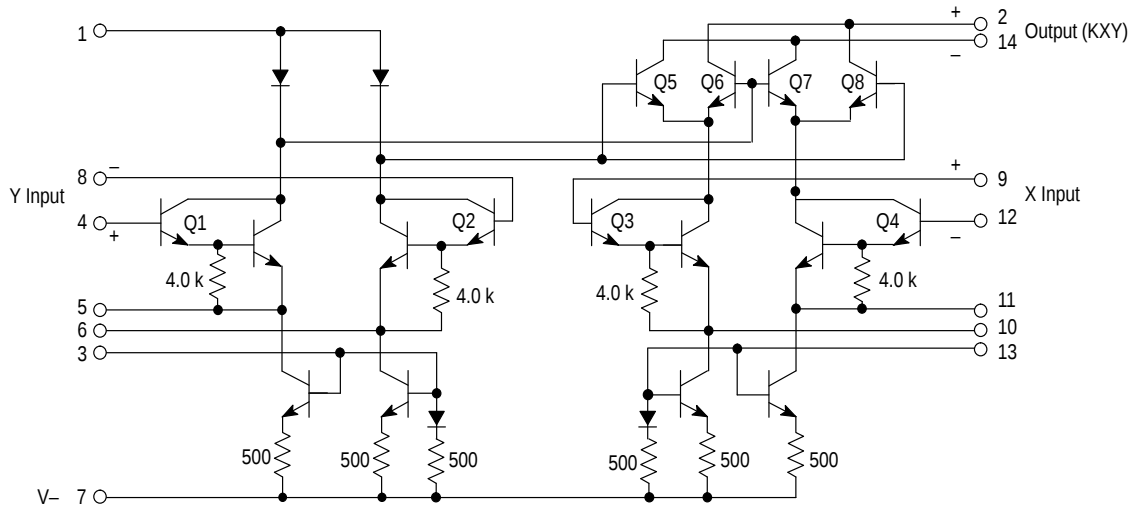
Figure 3. Circuit Schematic
