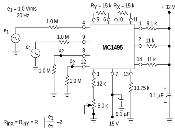
Figure 7. Input Resistance
