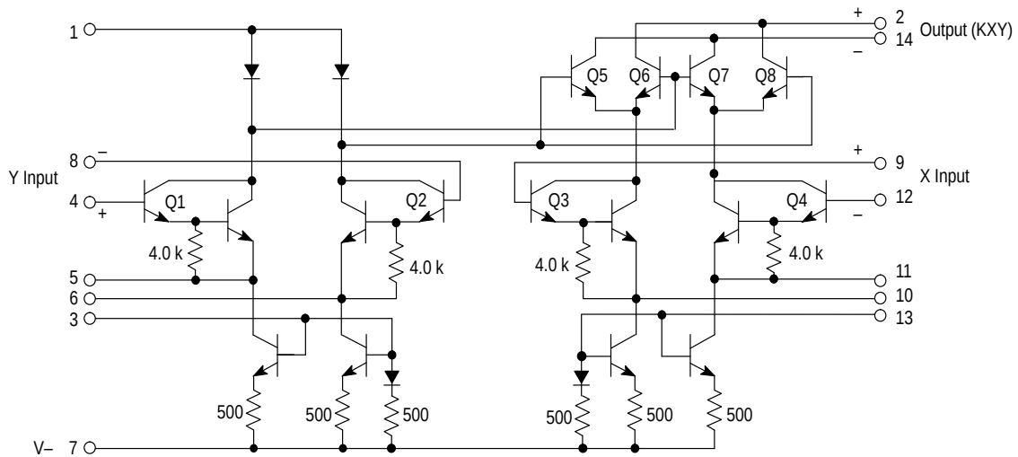
Figure 3. Circuit Schematic
