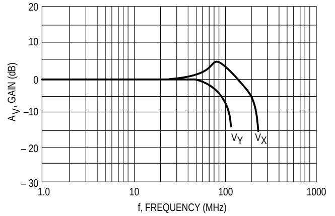
Figure 2. Transconductance Bandwidth
